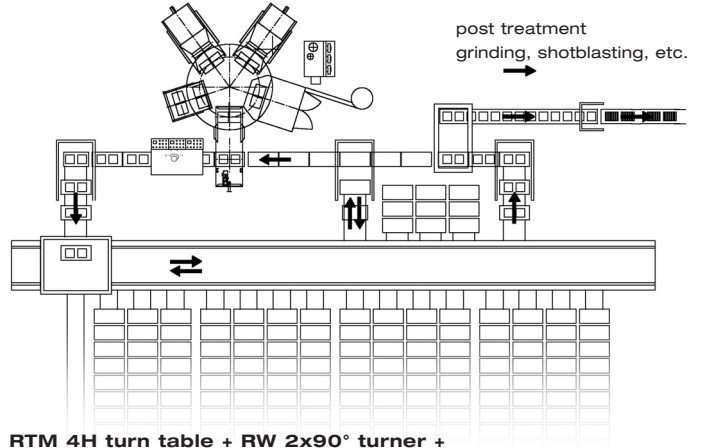
RTM 4H turn table + RW 2x90° turner + RFS flat stacking + RAS transfer car
