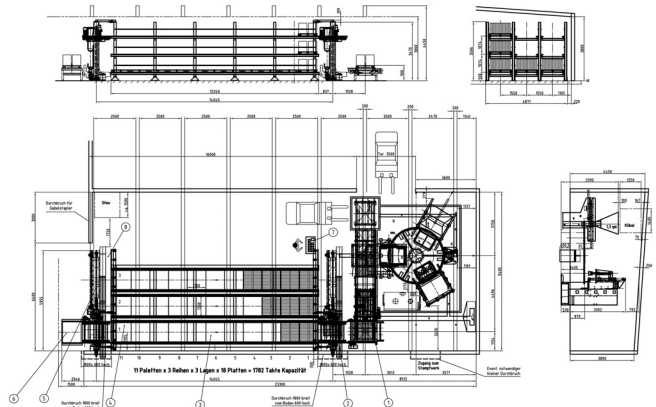
RTM 4H turn table + RAR automatic racking system
