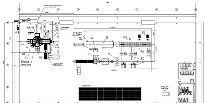
RTM 4H turn table + RSS edge stacking with forklift truck operation with additional splitting line
