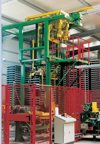
RTM 4H turn table + RW 2x90° turner + RFS flat stacking + RAS transfer car
