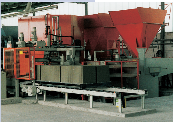
RTM 4H turn table + RSS edge stacking with forklift truck operation with additional splitting line
